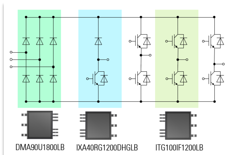
Figure 13. Power Section of an Inverter for Drives Application, Built by SMPD Devices
